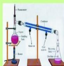
Distilation Apparatus Company : Borocil Glass Wear
