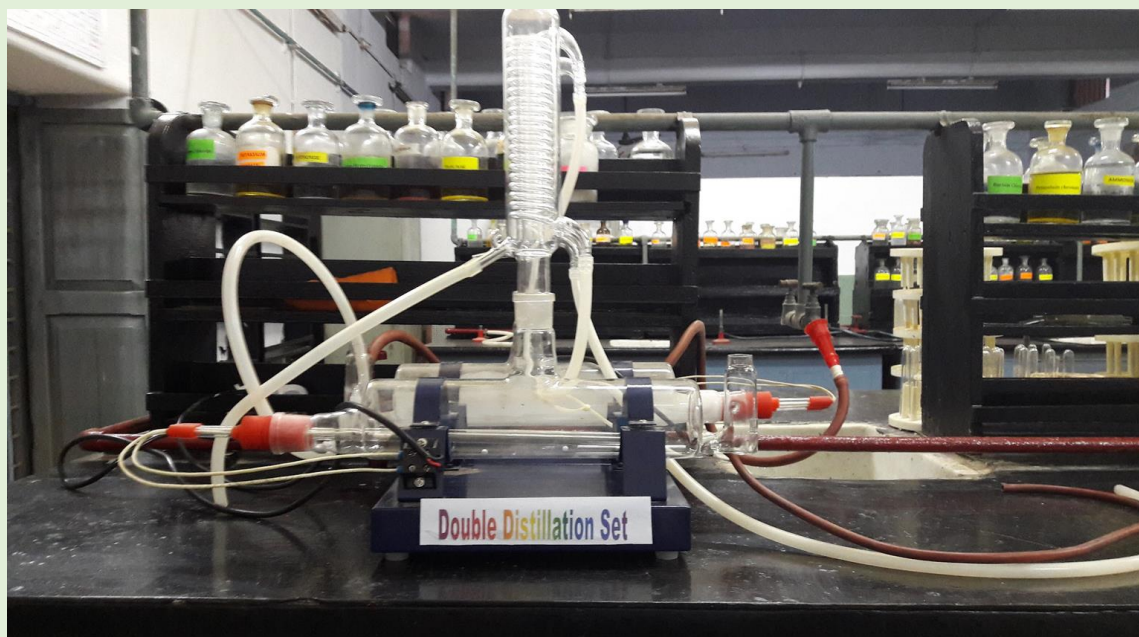
DOUBLE DISTILLATION SET
