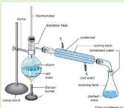
SIMPLE DISTILLATION APPARATUS
